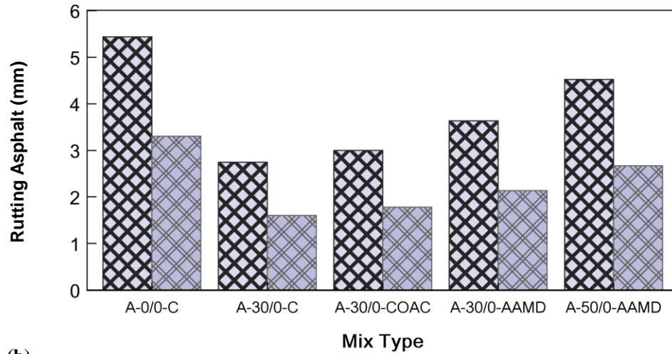
Figure 34. Pavement performance of the simulated pavement sections from Plant A: (a) bottom-up fatigue cracking and (b) asphalt rutting.
