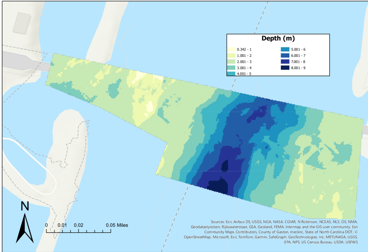
Figure 82: Depth measurements interpolated and smoothed.
