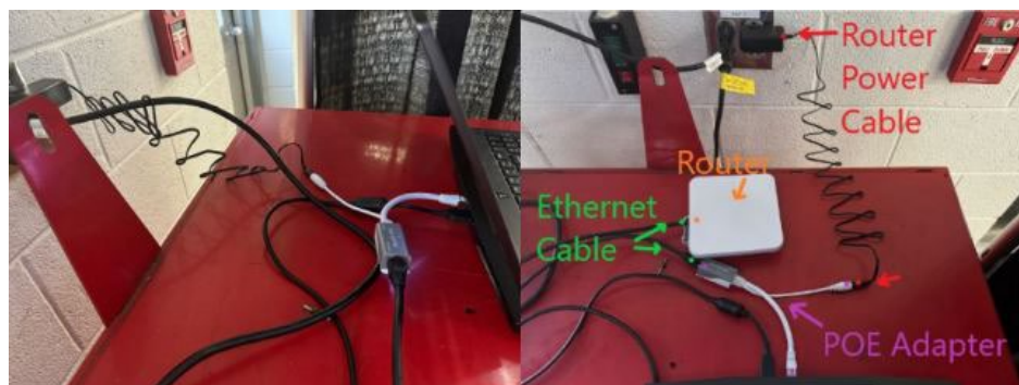
Figure 25: Connections required to remotely connect to ANP. In the field the router can be powered from a power bank.
