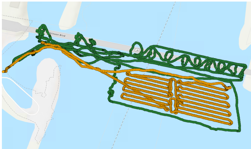
Figure 80: Two data collection runs were executed using the HyDrone USV. The first run (green markers) consisted of a remotely piloted survey in the vicinity of the bridge and an outline of a "box" in which to conduct the second automated survey (orange markers).
