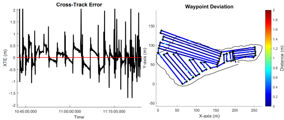
Figure 47: Cross-track error data from Test #12 in Mountain Island Lake (Left: cross-track error with time, Right: cross-track error overlaid on path).
