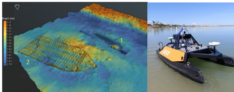
Figure 3. Example shipwreck data produced using HySweep module of the HYPACK software. Right: Data was collected using a Maritime Robotics Sea Otter USV equipped with a 700 kHz Norbit iWBMSe multibeam echosounder (Image Source: Solana et al, 2023)
