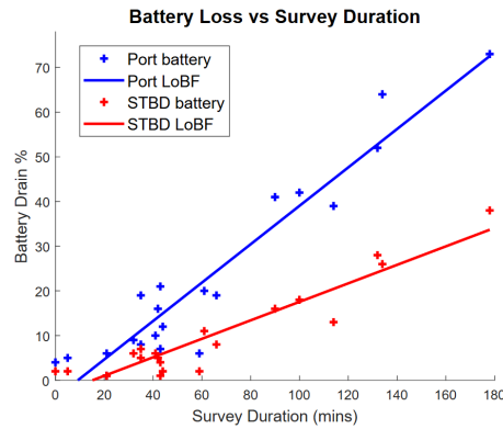
Figure 52: Battery drain percentage plotted against in-water survey duration.
