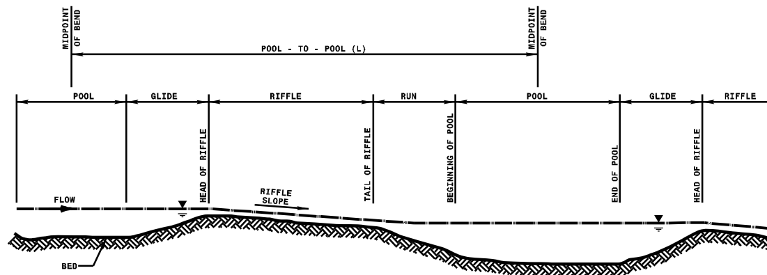
TYPICAL PROFILE
