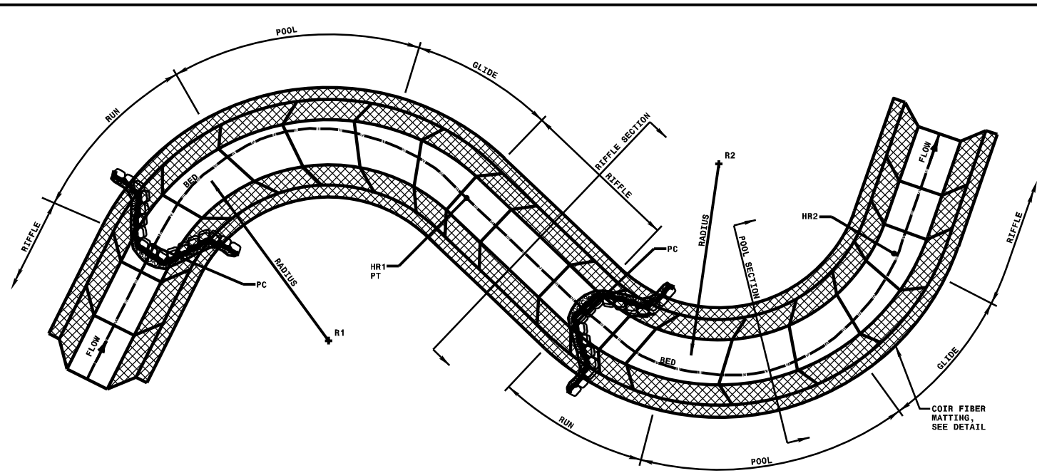
TYPICAL PLAN
