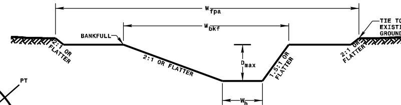
TYPICAL POOL WITH BANKFULL BENCH
