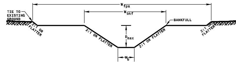
TYPICAL RIFFLE WITH BANKFULL BENCH
