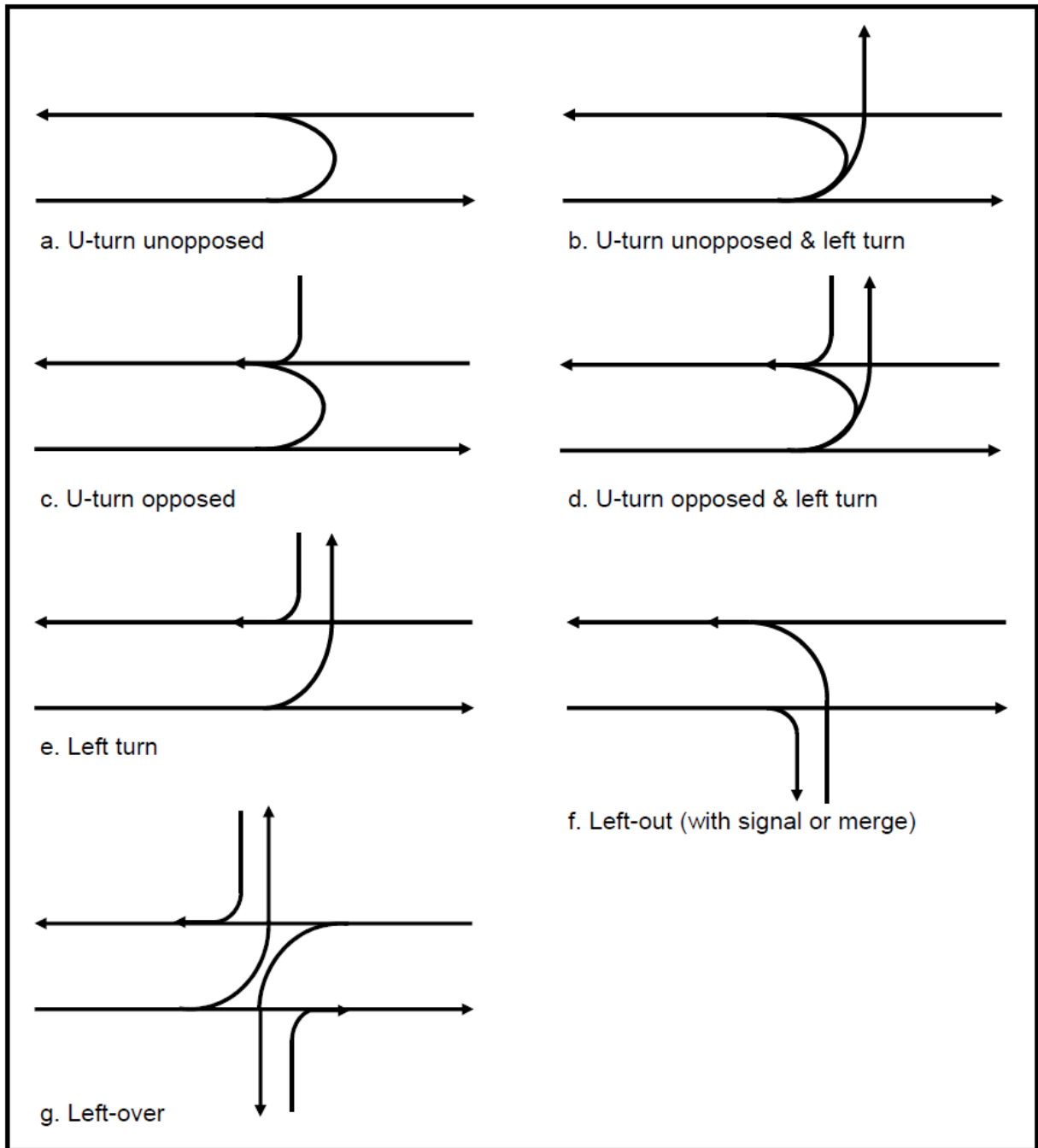
Figure 2.10. Crossover Types Considered for Saturation Flow Study
