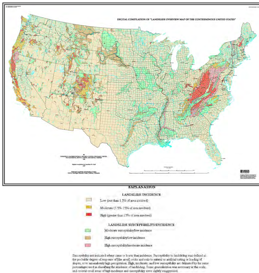
FIGURE 5.16: LANDSLIDE OVERVIEW MAP OF THE CONTERMINOUS UNITED STATES
