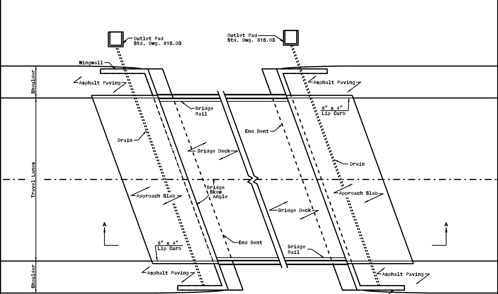
PLAN VIEW 12' APPROACH SLAB
