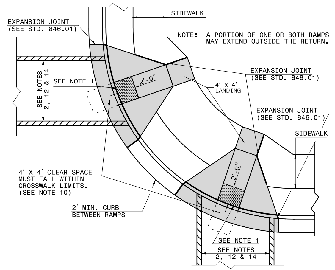
PLAN VIEW
