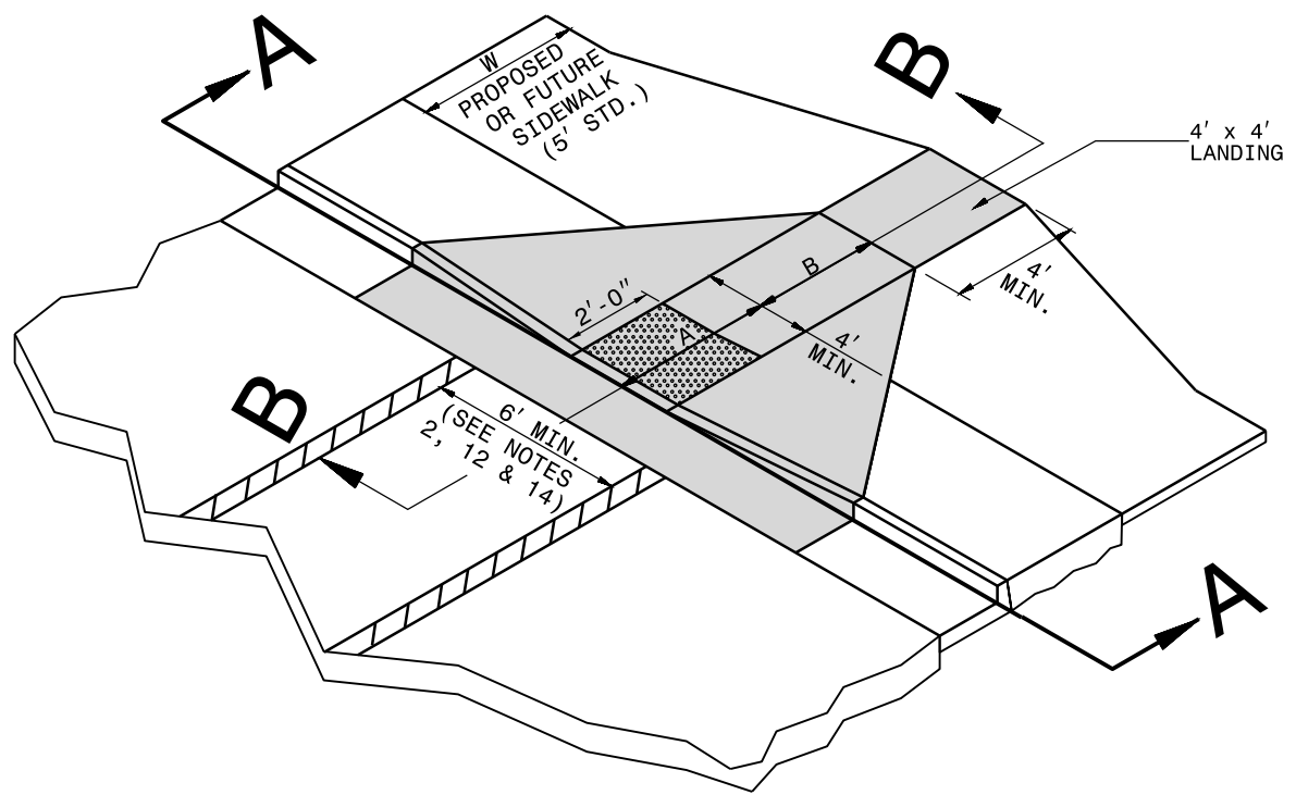
ISOMETRIC VIEW
