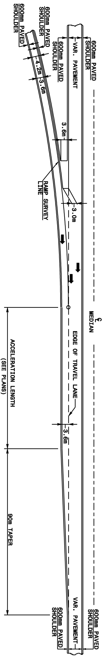
PARALLEL ENTRANCE FLEXIBLE PAVEMENT NON-INTERSTATE
