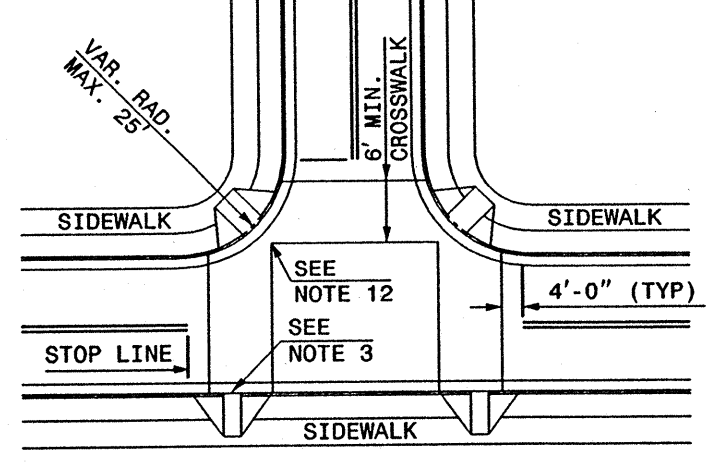
DETAIL SHOWING TYPICAL LOCATION OF WHEELCHAIR RAMP, PEDESTRIAN CROSSWALKS AND STOP LINES FOR TEE INTERSECTIONS
