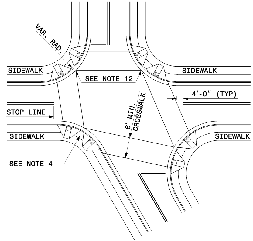
DETAIL SHOWING TYPICAL LOCATION OF WHEELCHAIR RAMP, PEDESTRIAN CROSSWALKS AND STOP LINES
