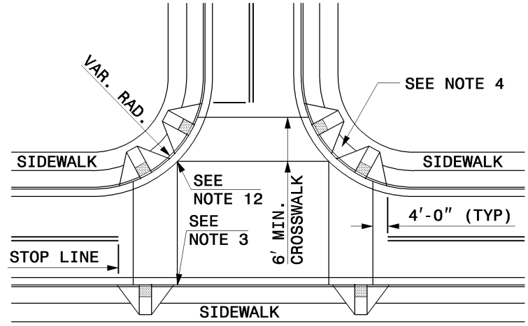
DETAIL SHOWING TYPICAL LOCATION OF WHEELCHAIR RAMP, PEDESTRIAN CROSSWALKS AND STOP LINES
