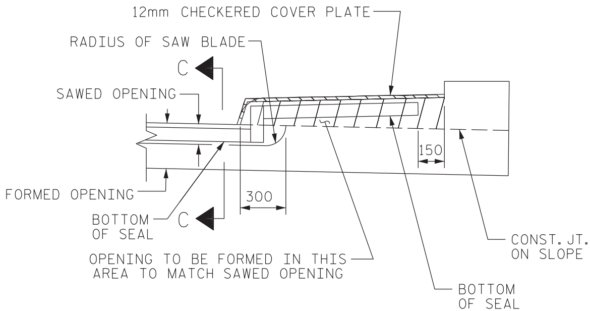
SECTION H-H
