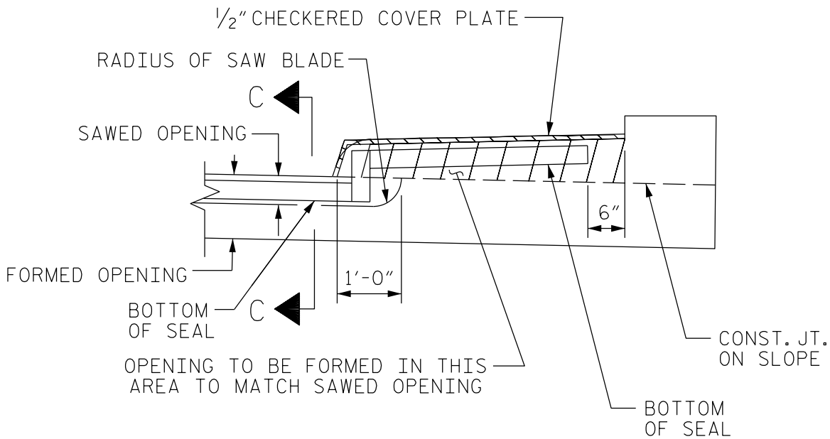
SECTION H-H
