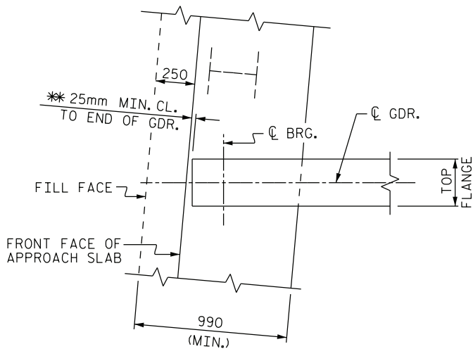
PLAN OF GIRDER AT INTEGRAL END BENT
