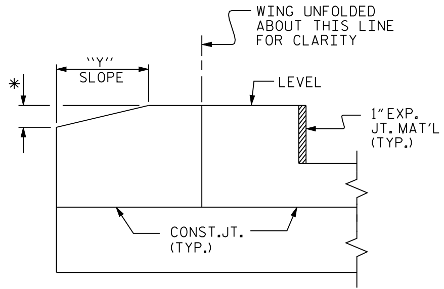
VIEW B-B
