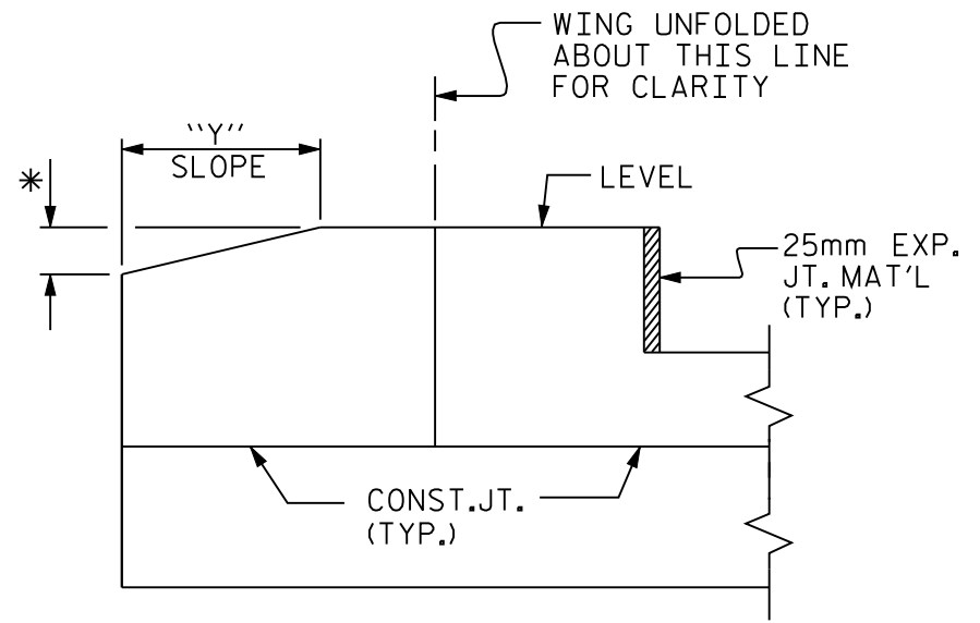
VIEW B-B
