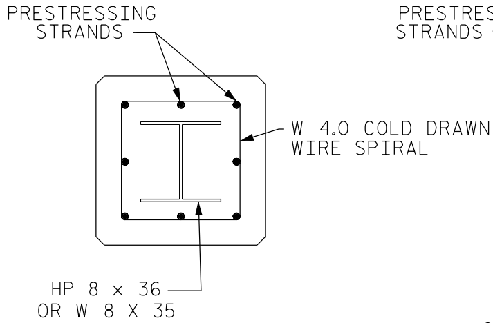
SECTION B-B FOR 16" SQUARE PRESTRESSED CONCRETE PILE
