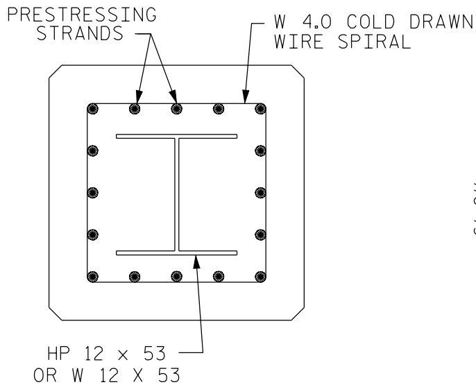
SECTION B-B FOR 24" SQUARE PRESTRESSED CONCRETE PILE
