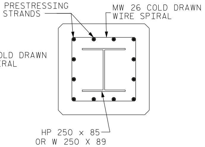
SECTION B-B FOR 508mm SQUARE PRESTRESSED CONCRETE PILE
