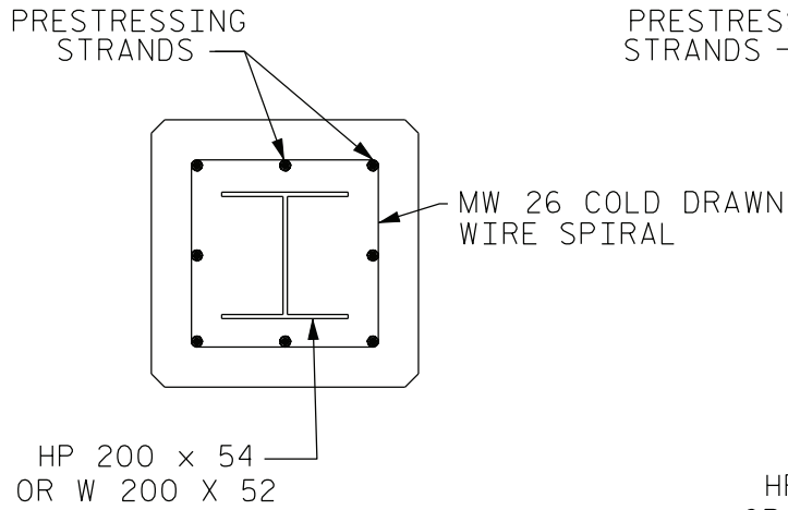
SECTION B-B FOR 406mm SQUARE PRESTRESSED CONCRETE PILE
