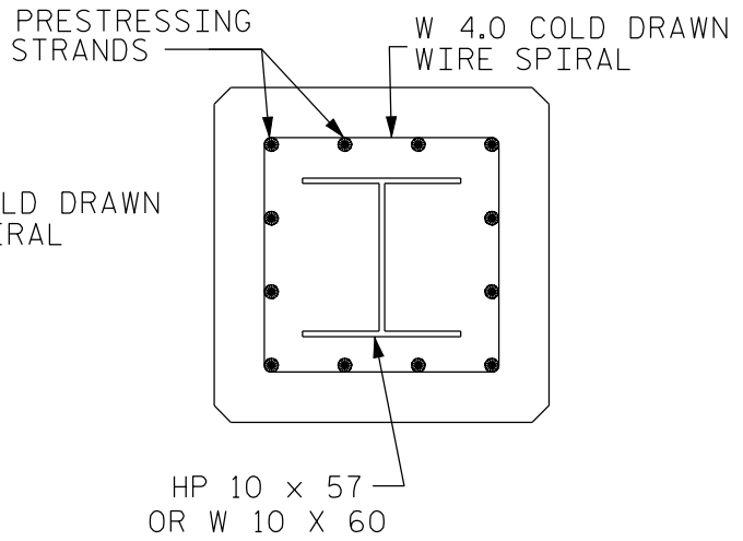
SECTION B-B FOR 20" SQUARE PRESTRESSED CONCRETE PILE
