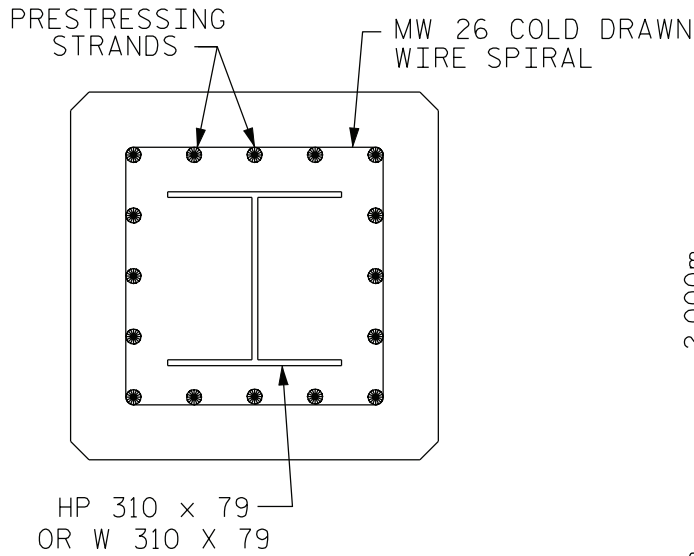
SECTION B-B FOR 610mm SQUARE PRESTRESSED CONCRETE PILE
