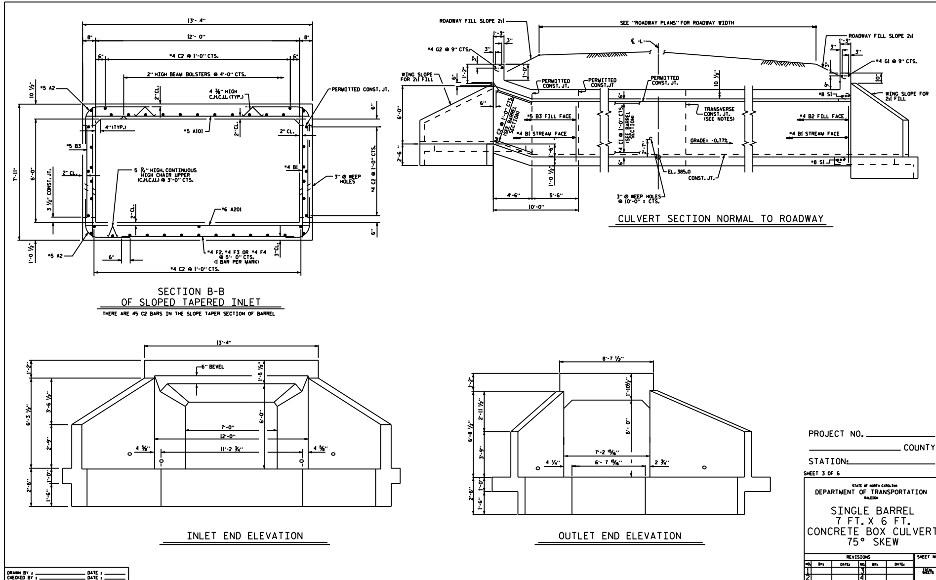
EXAMPLE OF SLOPED AND TAPERED INLET
