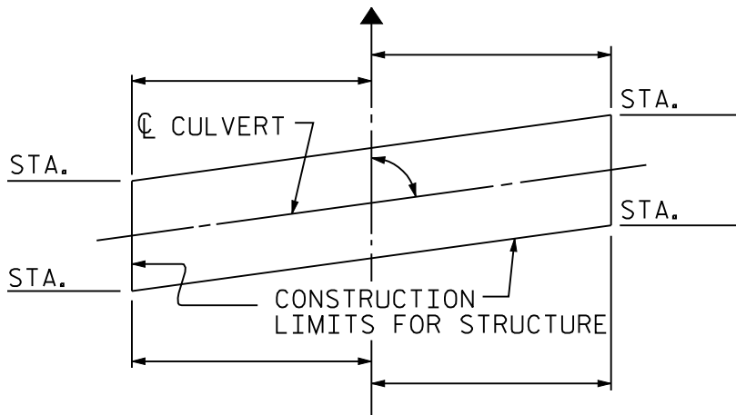
CONSTRUCTION LIMITS SKETCH FOR SKEWED CULVERT
