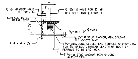
TYPICAL SECTION OF BASE ANGLE ASSEMBLY
