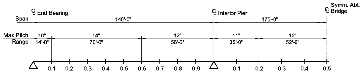
Figure 16: Shear Connector Pitch
