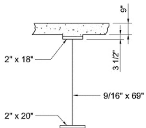
Figure 12: Section 2-2
