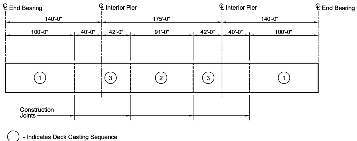
Figure 13: Deck-Placement Sequence
