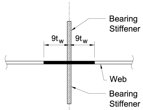
Figure 16: Effective Column Section for Bearing Stiffener Design
