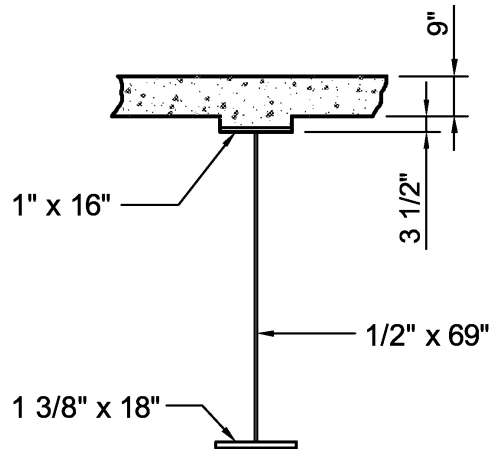
Figure 4: Preliminary Cross-Section - Positive Flexure
