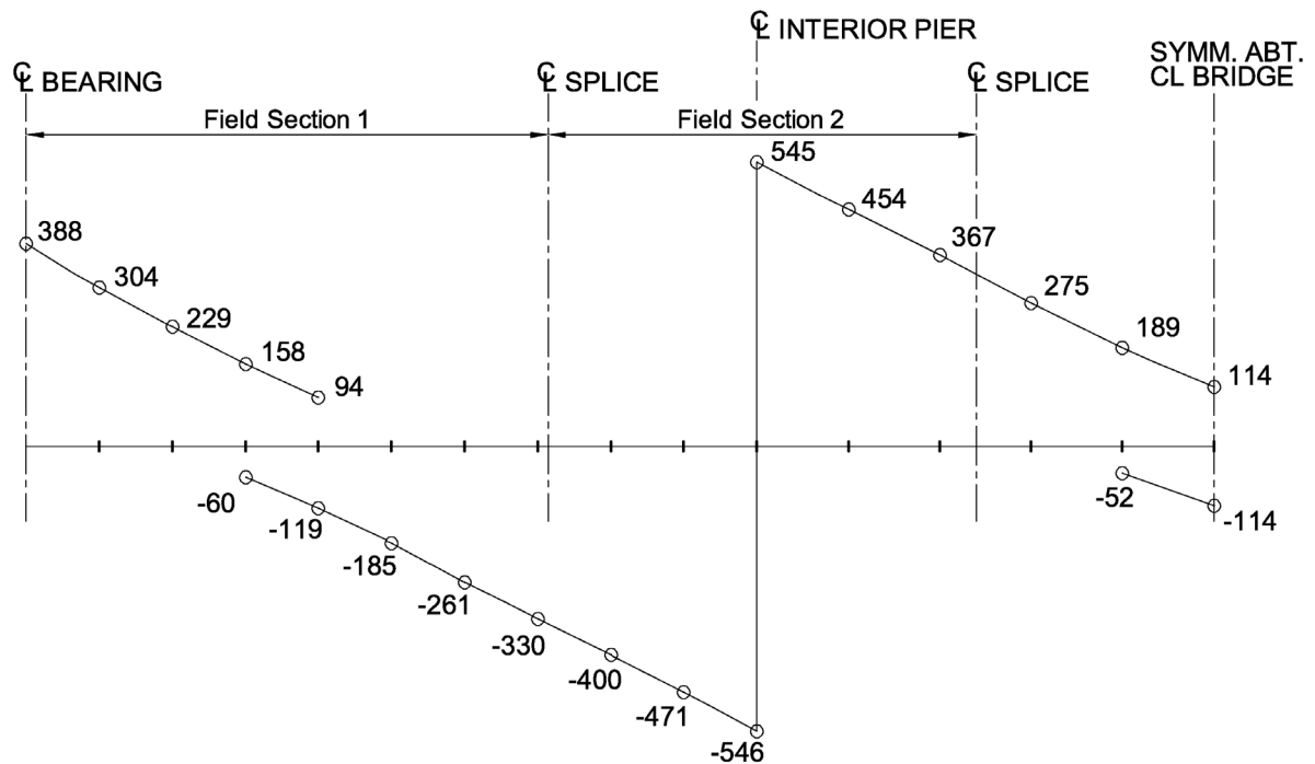
Figure 15: Design Shears Due to the Factored Loads - STRENGTH I
