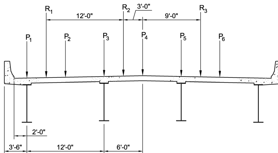
Figure 6: Exterior-Girder Distribution Factor - Special Analysis
