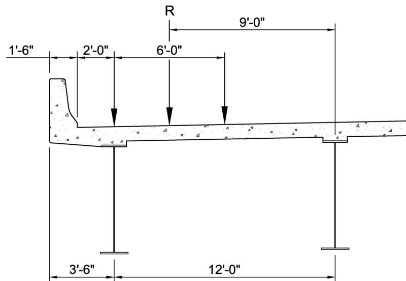
Figure 5: Exterior-Girder Distribution Factor - Lever Rule
