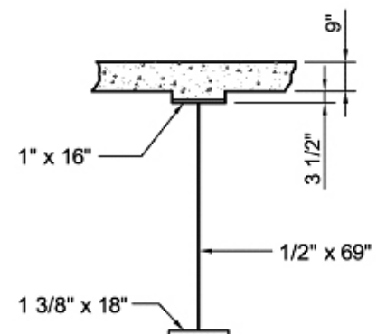
Figure 11: Section 1-1
