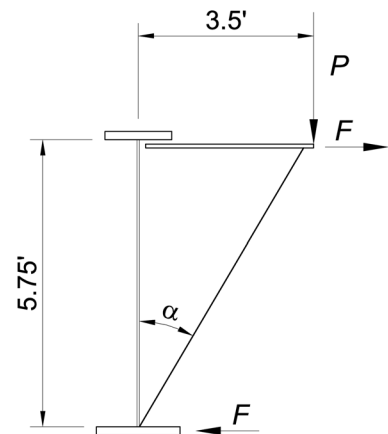
Figure 14: Deck Overhang Bracket
