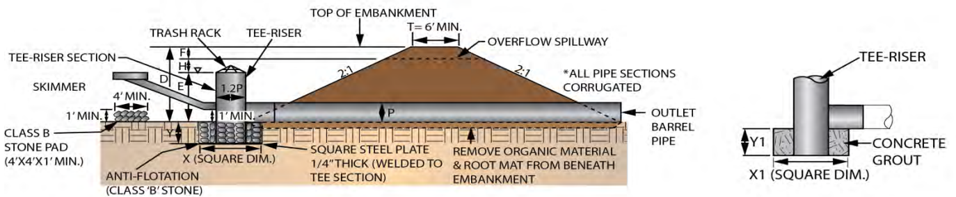
PROFILE VIEW (NOT TO SCALE)
