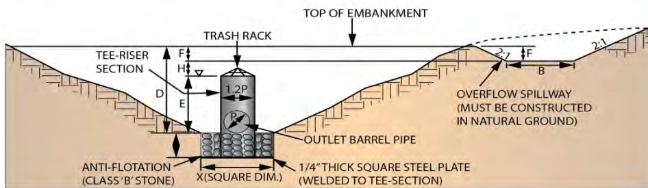
SECTIONAL VIEW (NOT TO SCALE)
