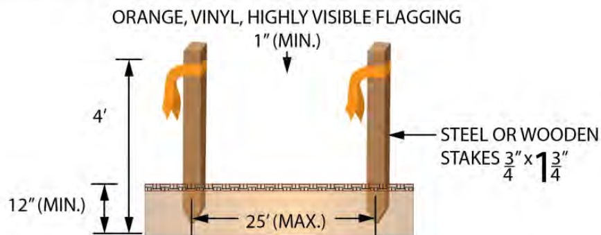
JURISDICTIONAL FLAGGING PLAN VIEW (NOT TO SCALE)
