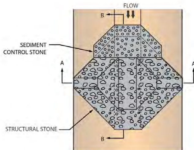
PLAN VIEW (NOT TO SCALE)
