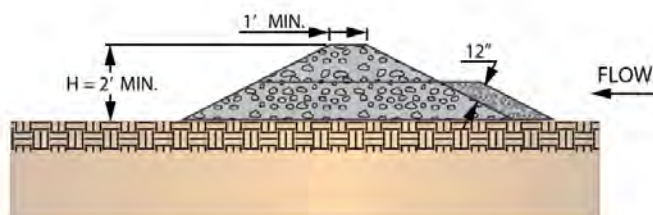
CROSS SECTION B-B (NOT TO SCALE)
