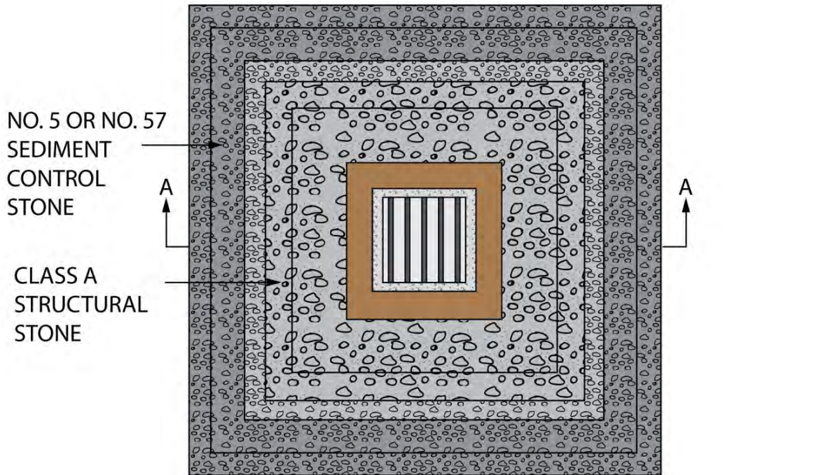
PLAN VIEW - TYPE B
