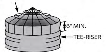
TRASH RACK DETAIL
