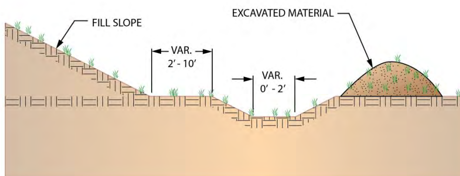
CROSS SECTION
