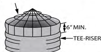
TRASH RACK DETAIL
