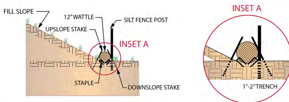
CROSS SECTION
