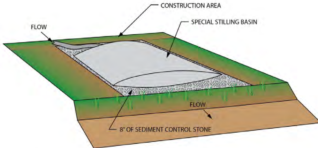
ISOMETRIC VIEW
