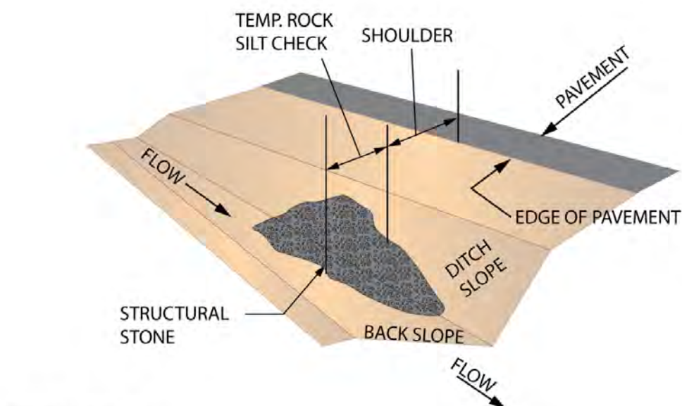
ISOMETRIC VIEW
