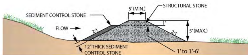
PROFILE SECTION - TYPE B
