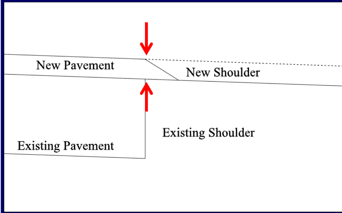
Cross Section 2 – Cross-Sectional Width Remains the Same
