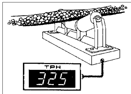
Figure 6-17 Weigh Bridge
