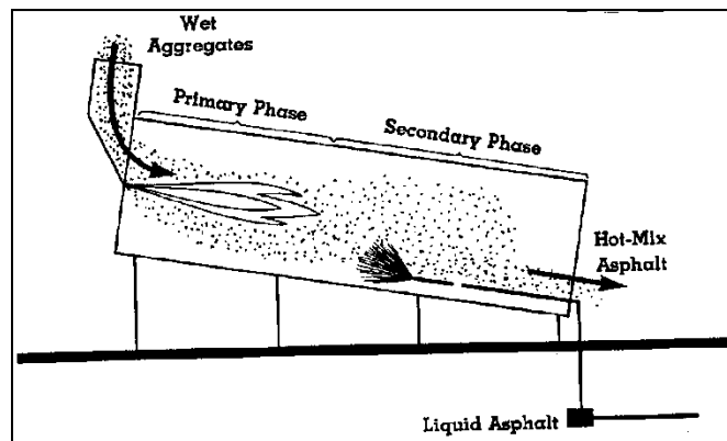
Figure 6-18 Zones in Drum Mixer
