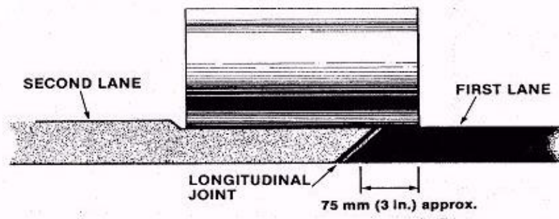
Figure 9-25 Joint Rolling Procedure
