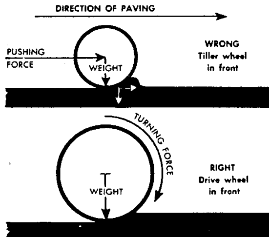
Figure 9-19 Forces Acting When Tiller Wheel or Drive Wheel is Forward
