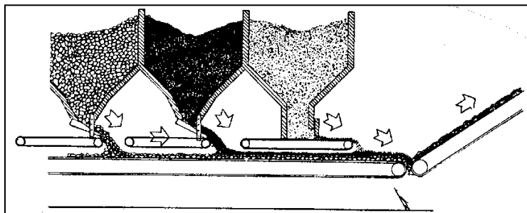
Figure 6-1 Three-Bin Cold Feeder and Belt
