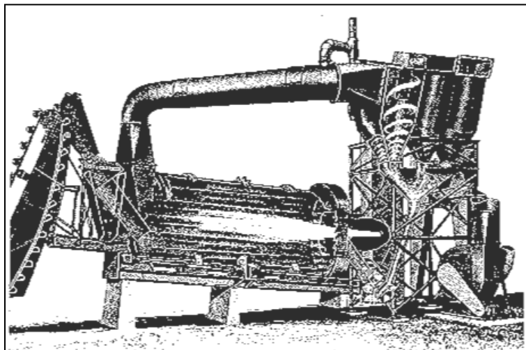
Figure 6-7 Dryer
