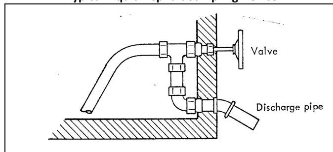
Figure 2-2 Typical Liquid Asphalt Sampling Device
