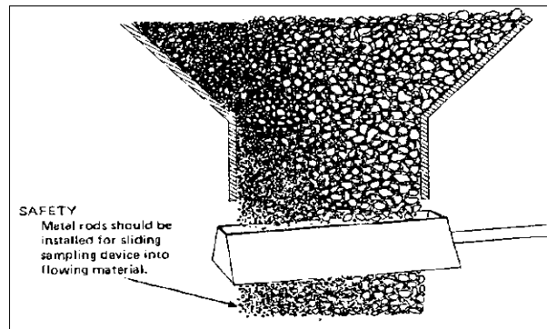
Figure 6-12 Correct Use of Sampling Device
