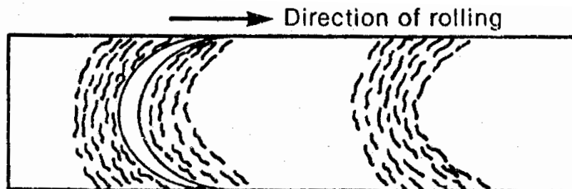
Figure 9-17 Heat Checking (Top View)
