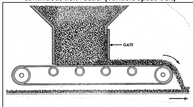
Figure 6-2 Continuous Belt Feeder (Variable Speed Belt)
