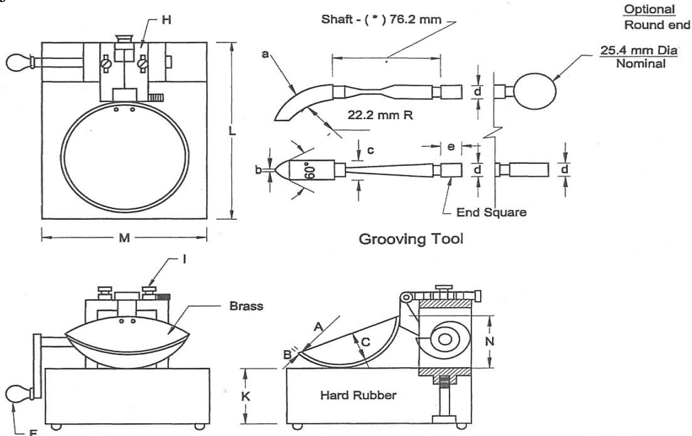
Figure 1 – Atterberg Device
