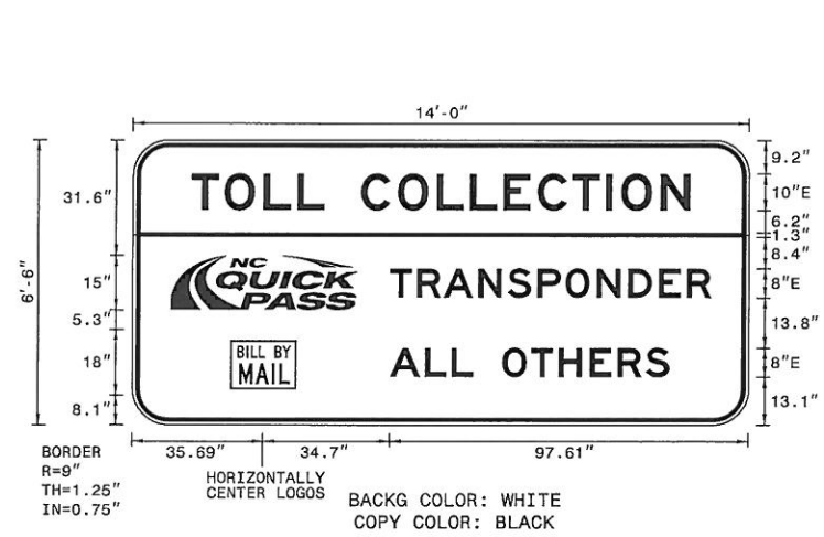
MAINLINE TOLL GANTRY SIGN PANELS
